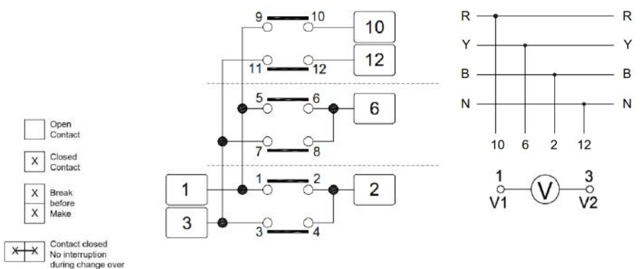
Wiring Diagram
