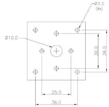
Drilling Plan
